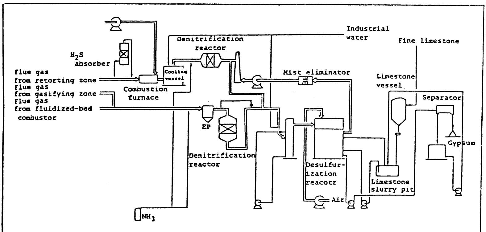
Fig. 7 Flow diagram of flue gas treatment process
