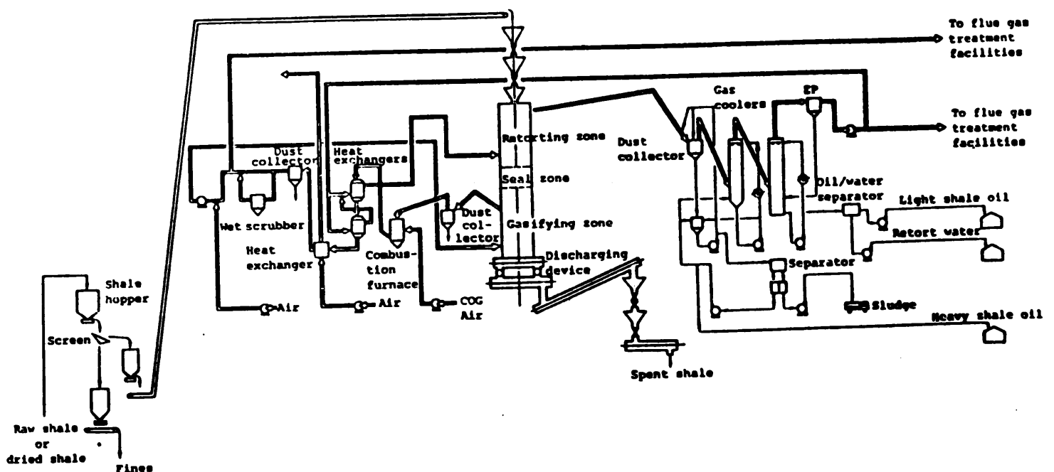
Fig. 5 Flow diagram of the retorting, gasifying, oil recovery and heat recovery processes
