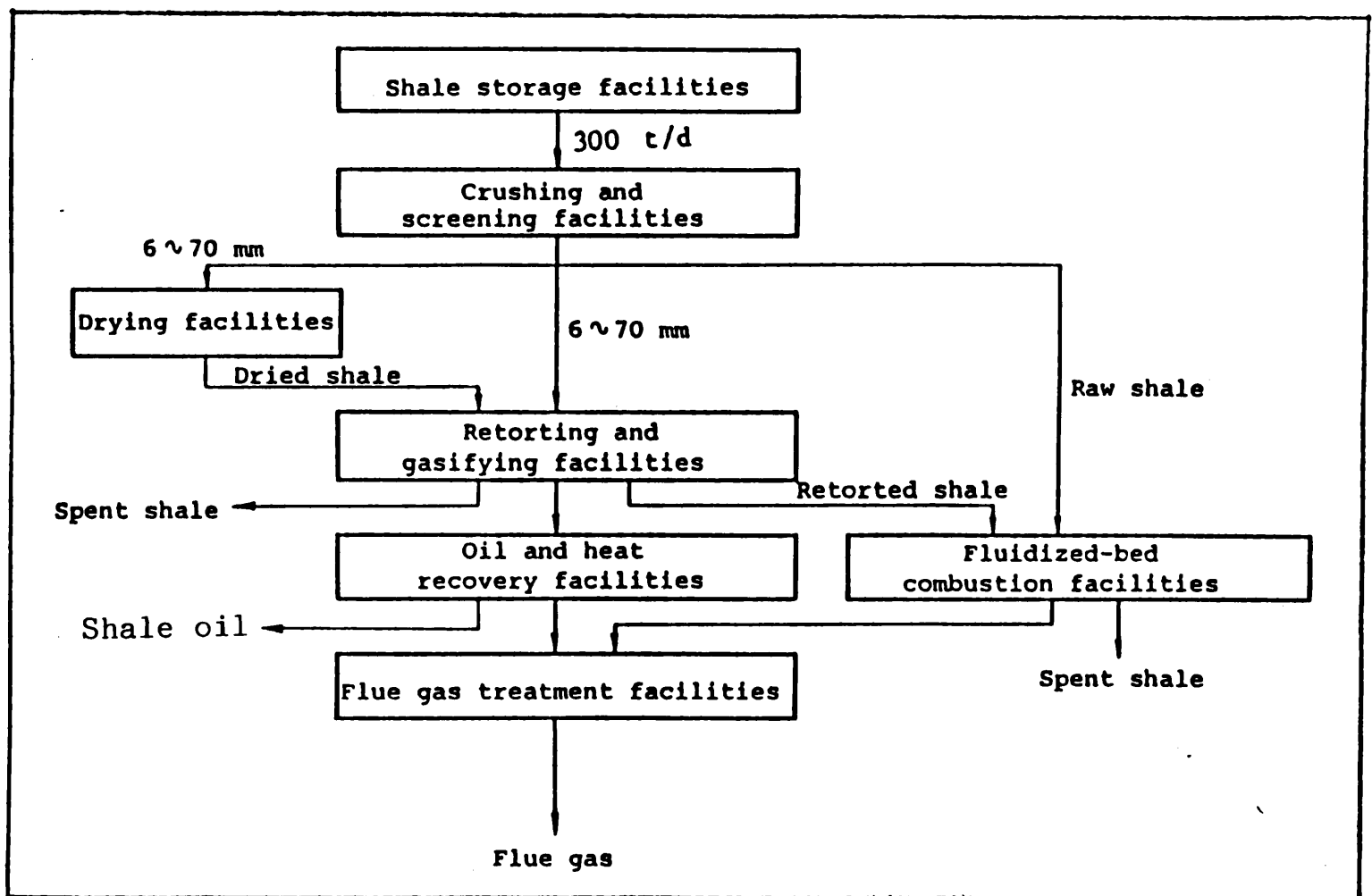
Fig. 1 Block diagram of pilot plant
