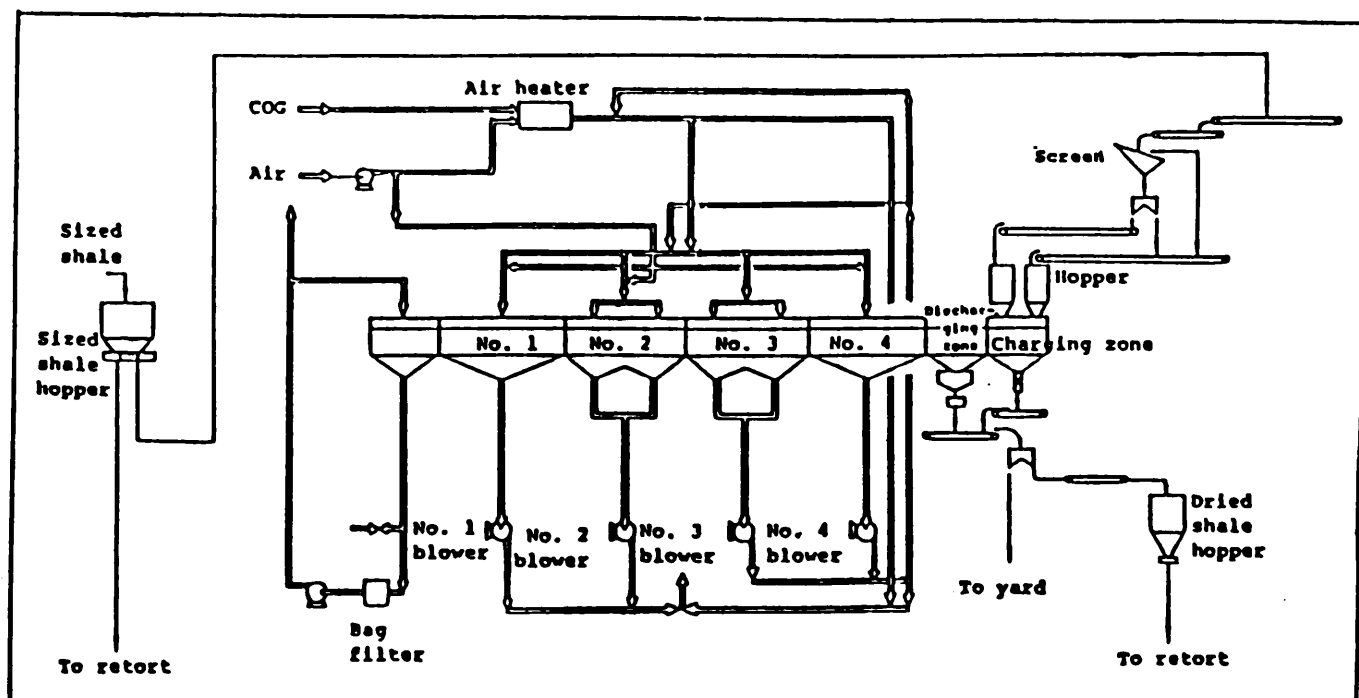
Fig. 3 Flow diagram of drying process
