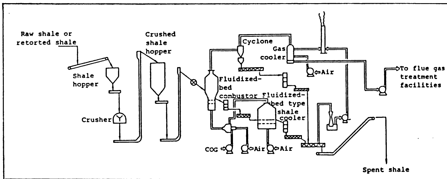
Fig. 6 flow diagram of fluidized-bed combustion process
